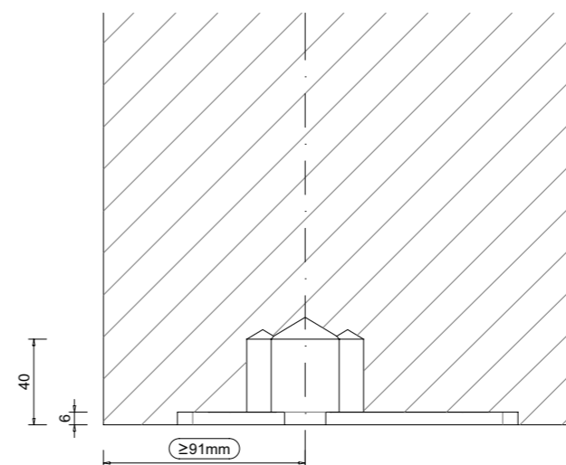
MILLING DRAWING
